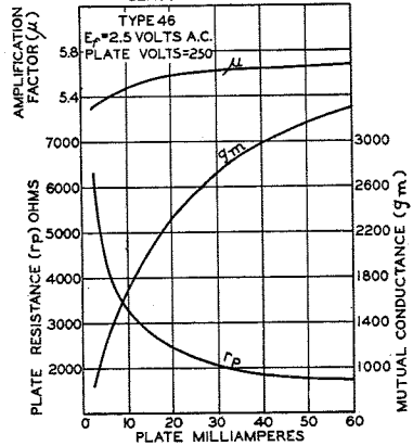
AVERAGE CHARACTERISTICS CLASS A OPERATION
