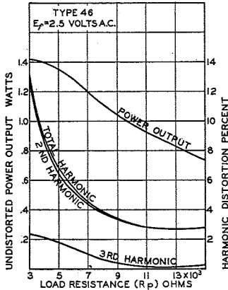
AVERAGE CHARACTERISTICS CLASS A OPERATION
