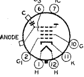
12C ANODE = G 4 + CL FOCUSING ELECTRODE = G 3
