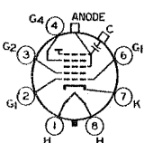
8BR ANODE = G 3 + G 5 + CL FOCUSING ELECTRODE = G 4
