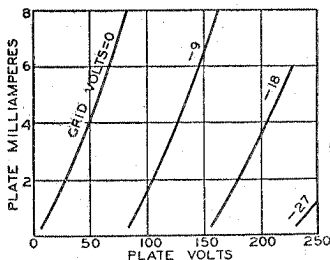
Fig. 12—Family of plate-characteristics curves.
