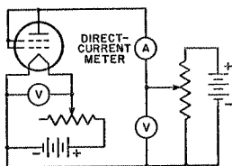
Fig. 130—Fundamental circuit of an emission tester
