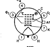
8KW ANODE = G 3 + G 5 + CL FOCUSING ELECTRODE = G 4
