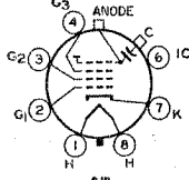
8JR ANODE = G 4 + CL FOCUSING ELECTRODE = G 3
