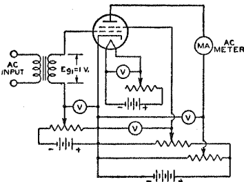
Fig. 132—Fundamental circuit of a dynamic transconductance tester.
