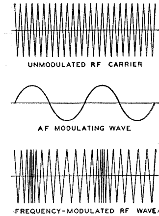
Fig. 28—Waveforms showing effect of frequency modulation on an rf wave.
