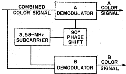
Fig. 94—Separation of combined color signal into two signals at the receiver.
