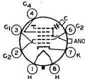
8JK ANODE = G 3 + G 5 + CL FOCUSING ELECTRODE = G 4
