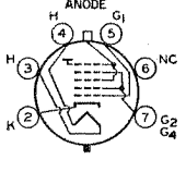
7FG ANODE = G 3 + G 5 + CL AUTOMATIC FOCUSING
