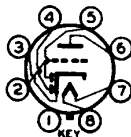
BOTTOM VIEW (8Q)
